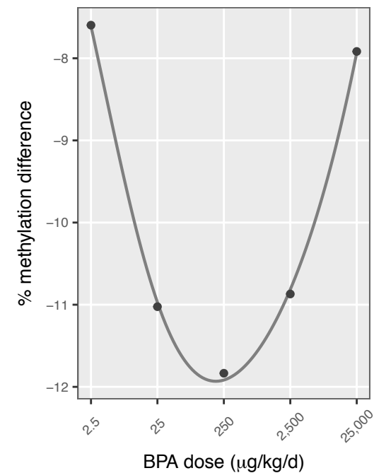
24 chr4: 157,585,001
