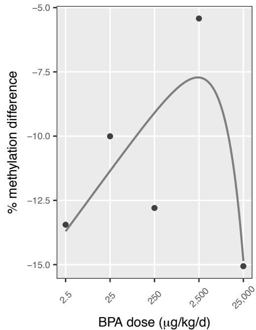
5 chr10: 104,079,501
