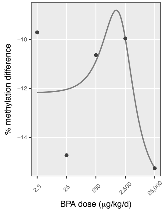
29 chr7: 141,375,801
