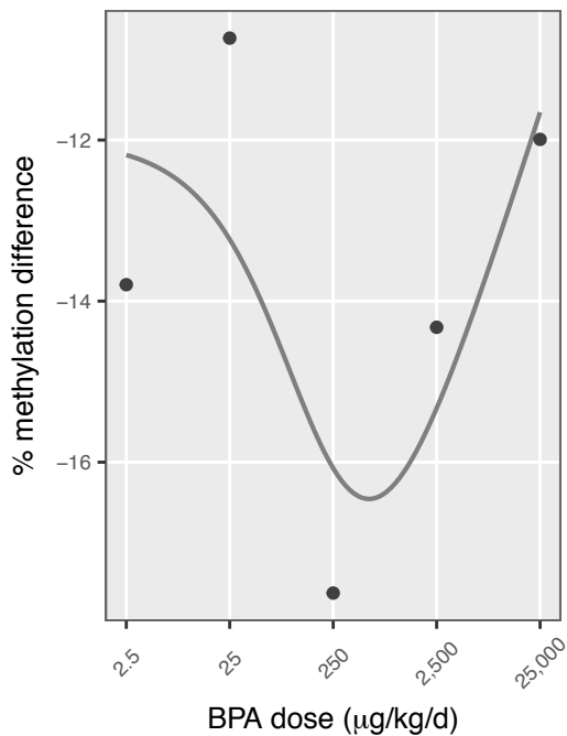
22 chr20: 45,282,001
