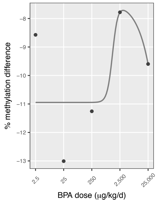
13 chr12: 22,137,001
