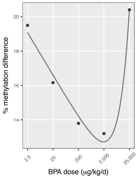
14 chr12: 22,882,301
