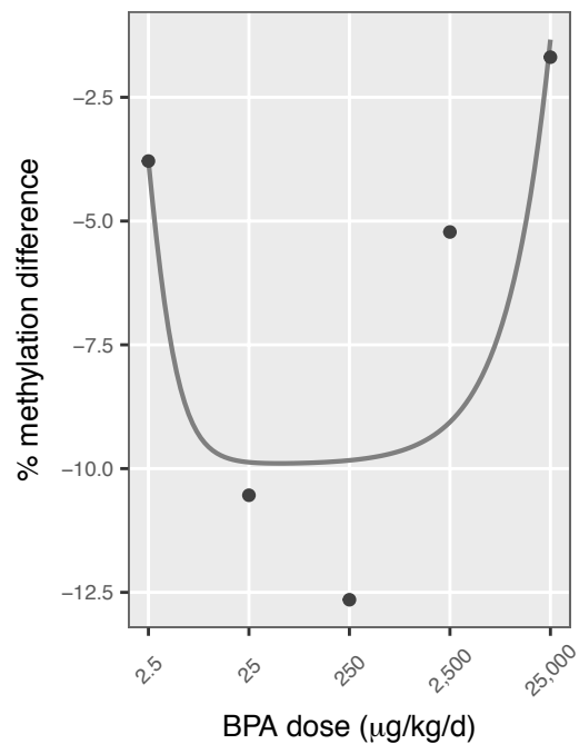
21 chr20: 14,469,401
