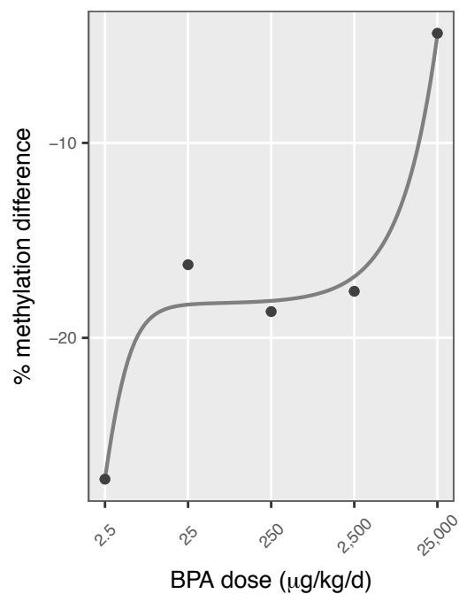
7 chr10: 105,102,101
