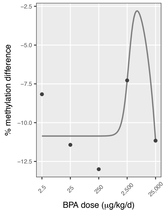
15 chr12: 39,836,101
