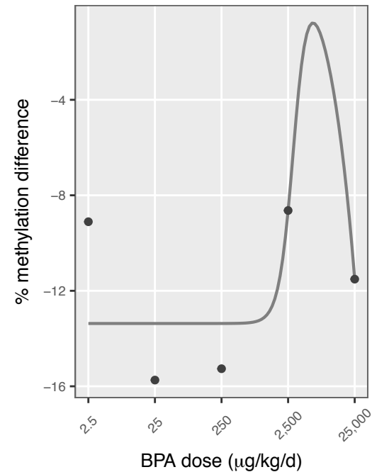
32 chr9: 65,763,501
