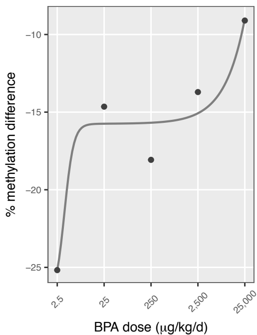
6 chr10: 105,102,001
