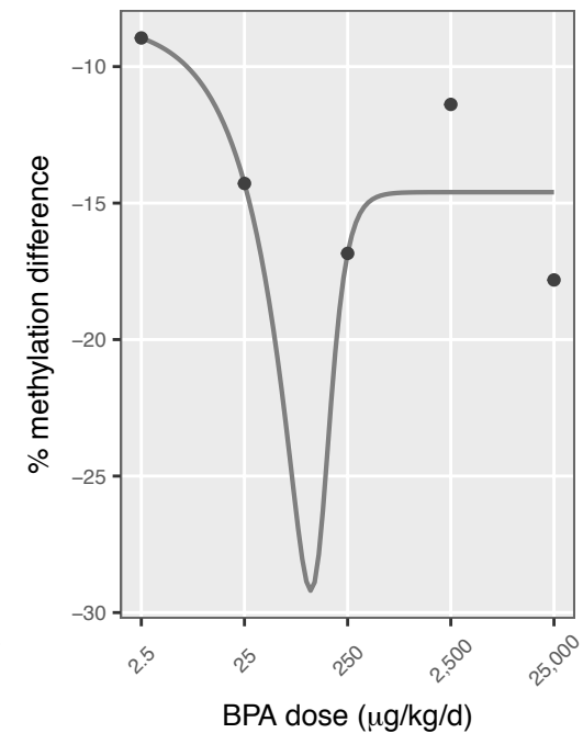
16 chr12: 44,231,401
