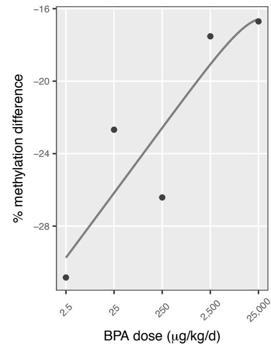
8 chr10: 105,102,901
