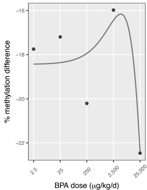
23 chr3: 12,610,501
