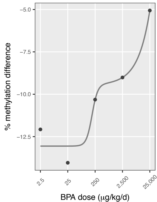
7 chr10: 105,102,101
