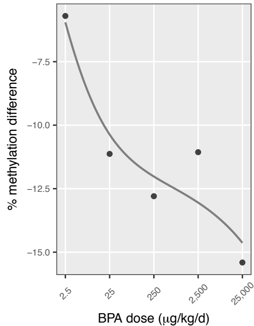
31 chr8: 130,402,401
