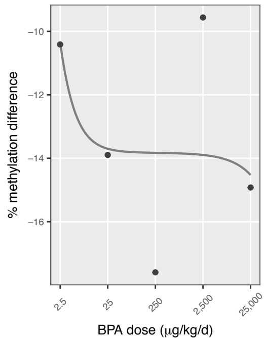
5 chr10: 104,079,501
