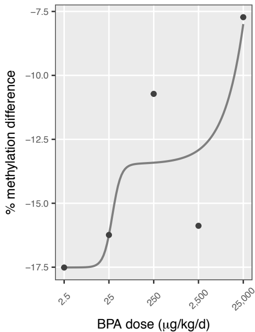
6 chr10: 105,102,001
