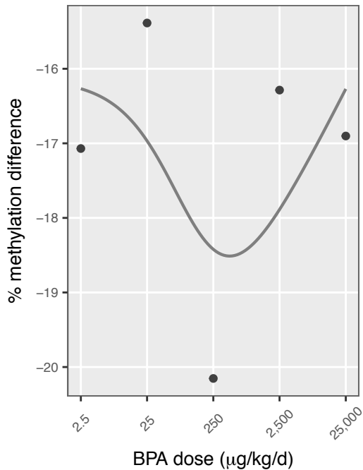
30 chr8: 130,402,101
