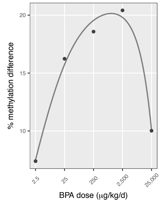
8 chr10: 105,102,901
