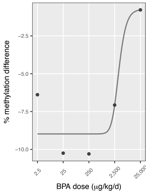
22 chr20: 45,282,001
