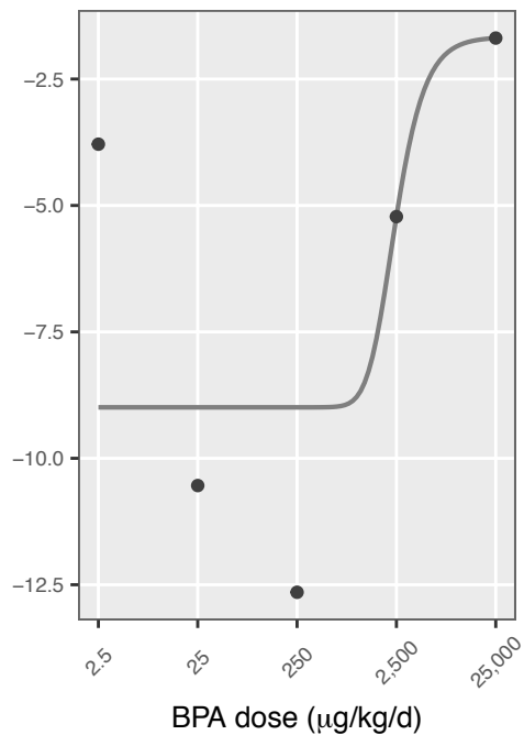
21 chr20: 14,469,401
