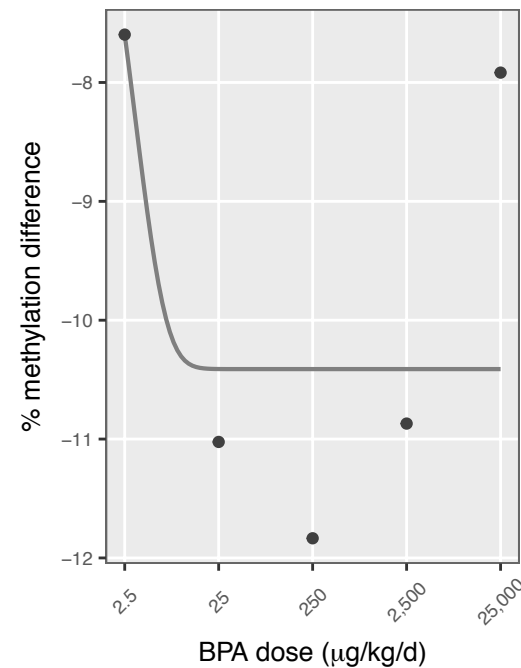
24 chr4: 157,585,001
